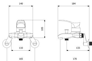
BS2-1-6001 샤워기
