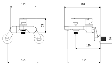
By - 6001 샤워기
